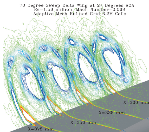
Fig. 12 Cross planes of vorticity at four streamwise stations (300, 325, 350, and 375 mm) for the AMR grid detached-eddy simulation demonstrating the vortical substructures captured with CFD.
