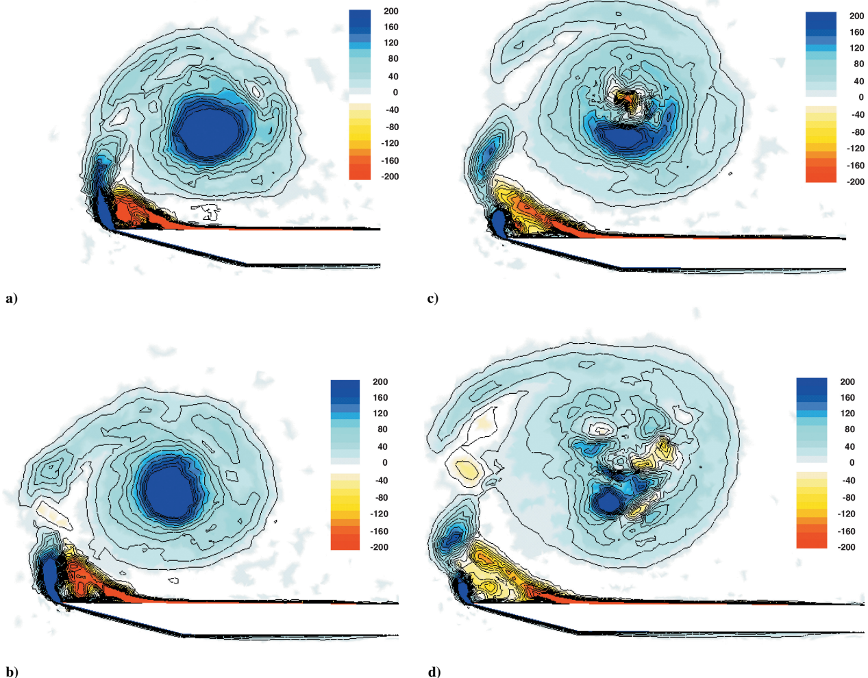
Fig. 10 Grid 4 detached-eddy-simulation results of instantaneous axial vorticity ( \Omega_x c/U_\infty ) at \alpha = 27 deg and U_\infty = 24 m/s: a) X/c = 0.53 (500 mm), b) X/c = 0.63 (600 mm), c) X/c = 0.74 (700 mm), and d) X/c = 0.84 (800 mm).
